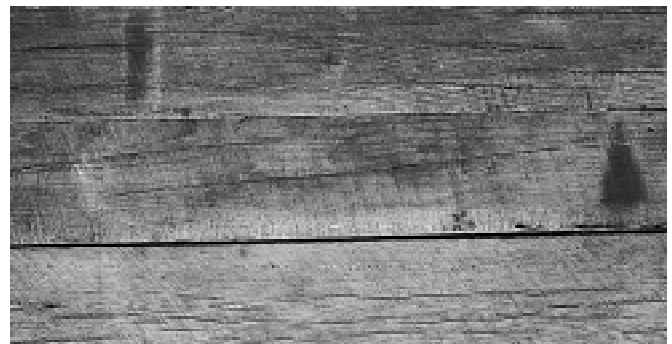
Figure 48—These oak boards surface checked in the early stages of air drying. These surface checks can penetrate deep into the wood, and when they close at the surface, the internal failure appears to be honeycomb.
